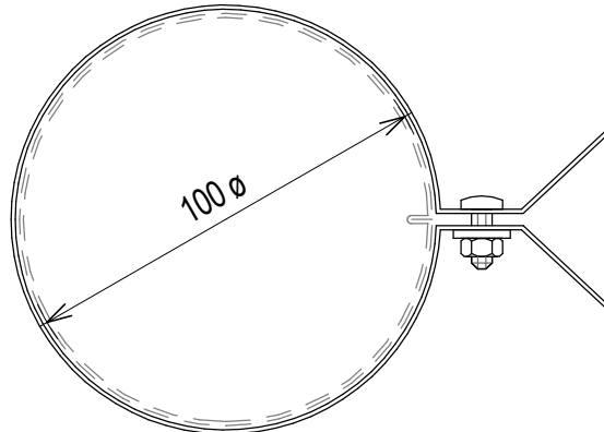
CG 100ø Downpipe Clip
