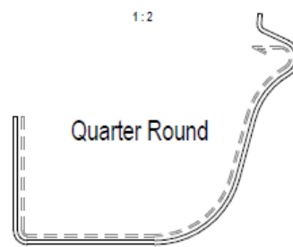
135mm Quarter Round External Bracket 1:2
