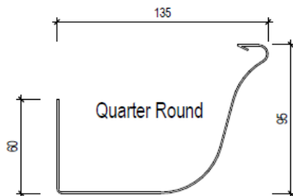
135mm Quarter Round
