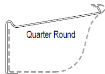
135mm Quarter Round Internal Bracket 1:2
