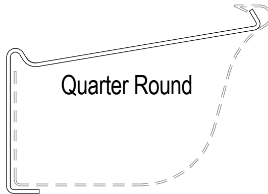
135mm Quarter Round Internal Bracket 1:2
