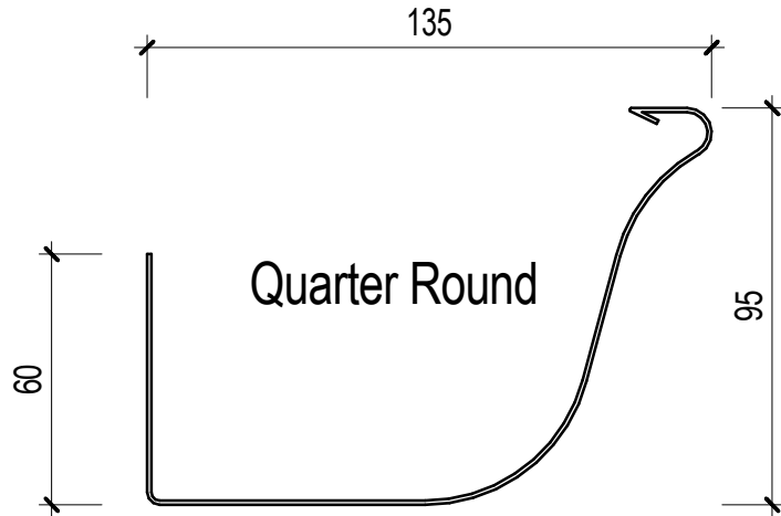
135mm Quarter Round 1:2
